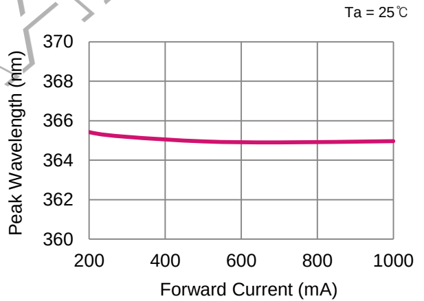
■ Forward Current vs. Peak Wavelength
