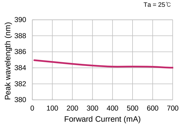
■ Forward Current vs. Peak Wavelength
