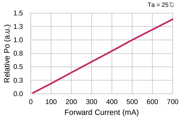
■ Forward Current vs. Relative Radiant Flux
