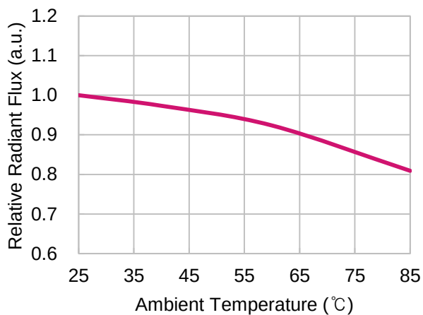
■ Derating Curve
